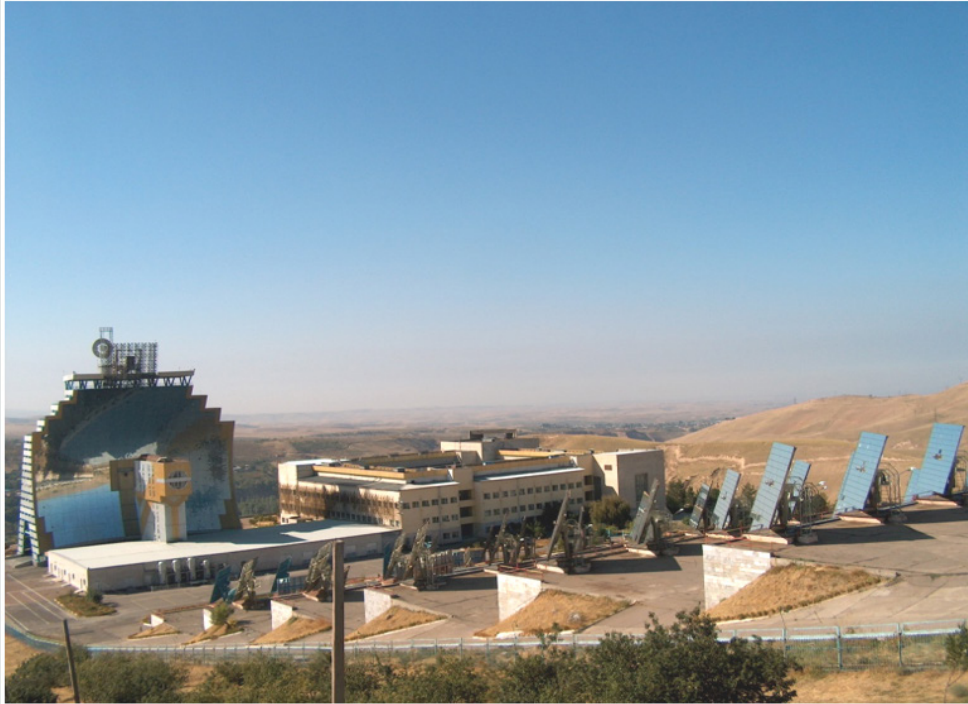
Figure 1: Big solar furnace with the power of 1000 kilowatt Scientific-industrial association “Physics-Sun” Academy of Sciences of the Republic of Uzbekistan.
