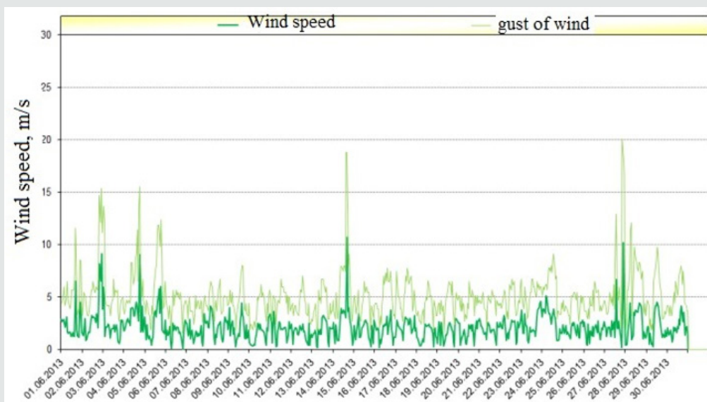
Figure 3: Gust and hourly averaged wind speed values measured by the Parkent weather station MHP MS4-12-1 in the month of June 2013.
