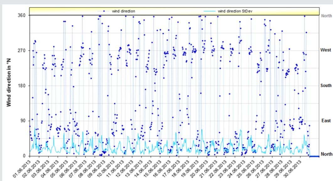
Figure 4: Wind directions measured by the Parkent weather station MHP MS4-12-1 in the month of June 2013 (wind direction - wind direction relative to the north, wind direction StDev - standard deviation of the change in wind direction within the measurement interval in degrees).
